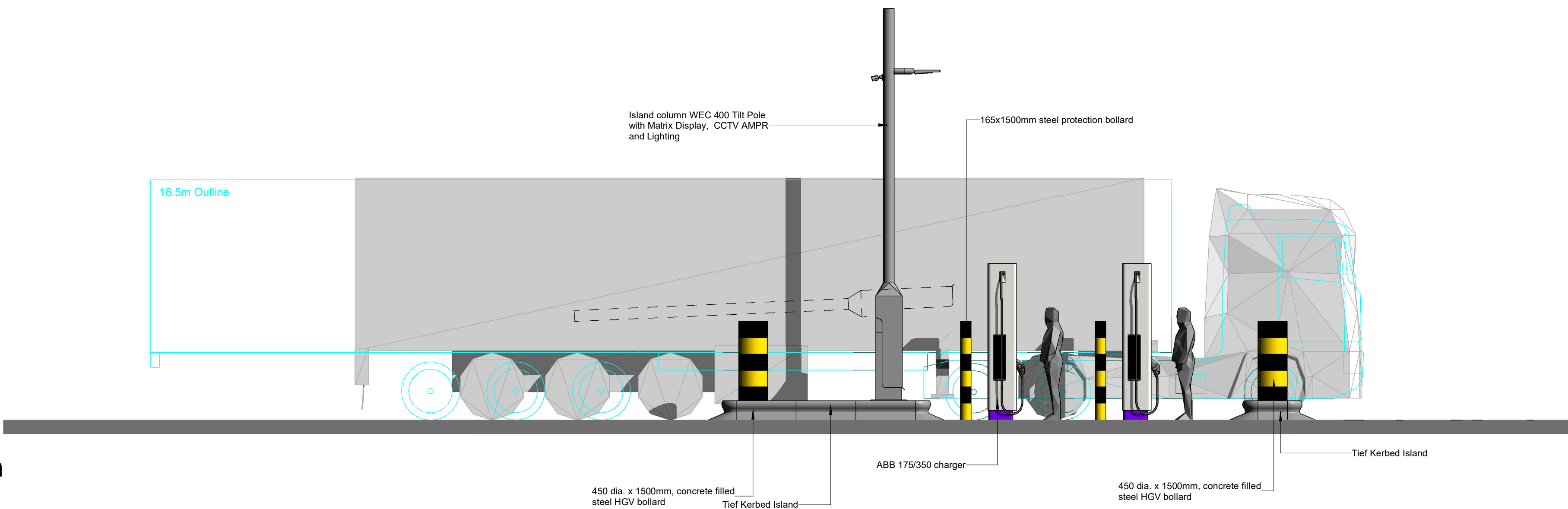
Straight Through Bay - Right Side Elevation 1 : 50
