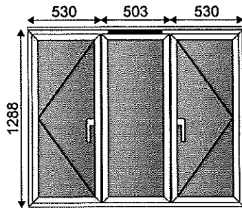
1 - 1563w x 1288h (Basic Frame Size) 1 - 1563w x 1308h Viewed Outside
