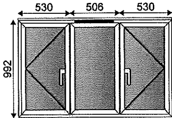
1 - 1566w x 992h (Basic Frame Size) 1 - 1566w x 1012h Viewed Outside
