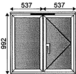
1 - 1074w x 992h (Basic Frame Size) 1 - 1074w x 1012h Viewed Outside
