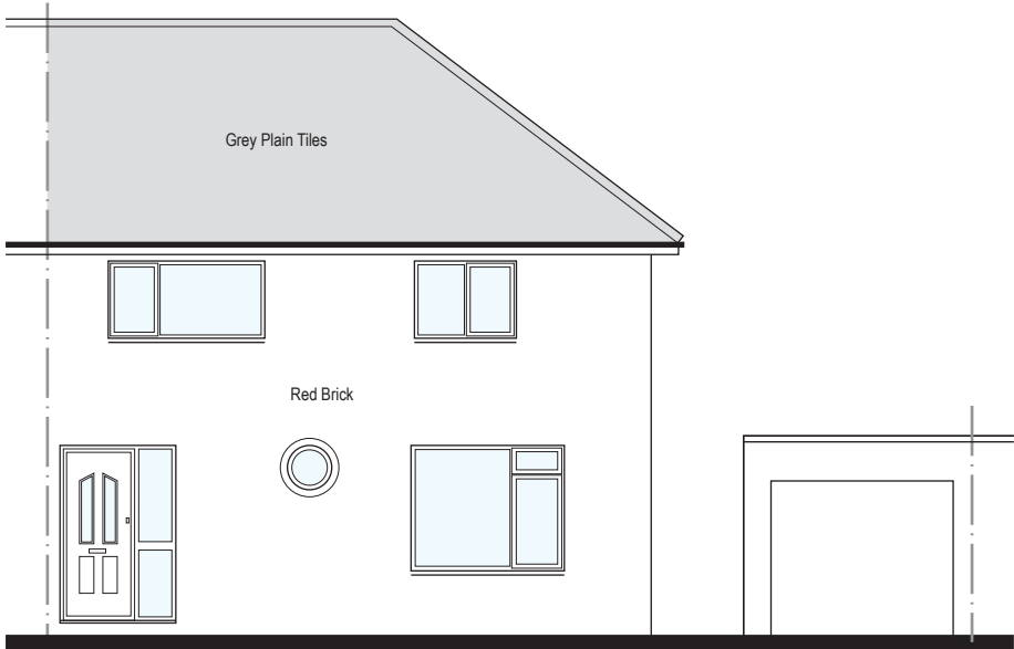
Front Elevation
