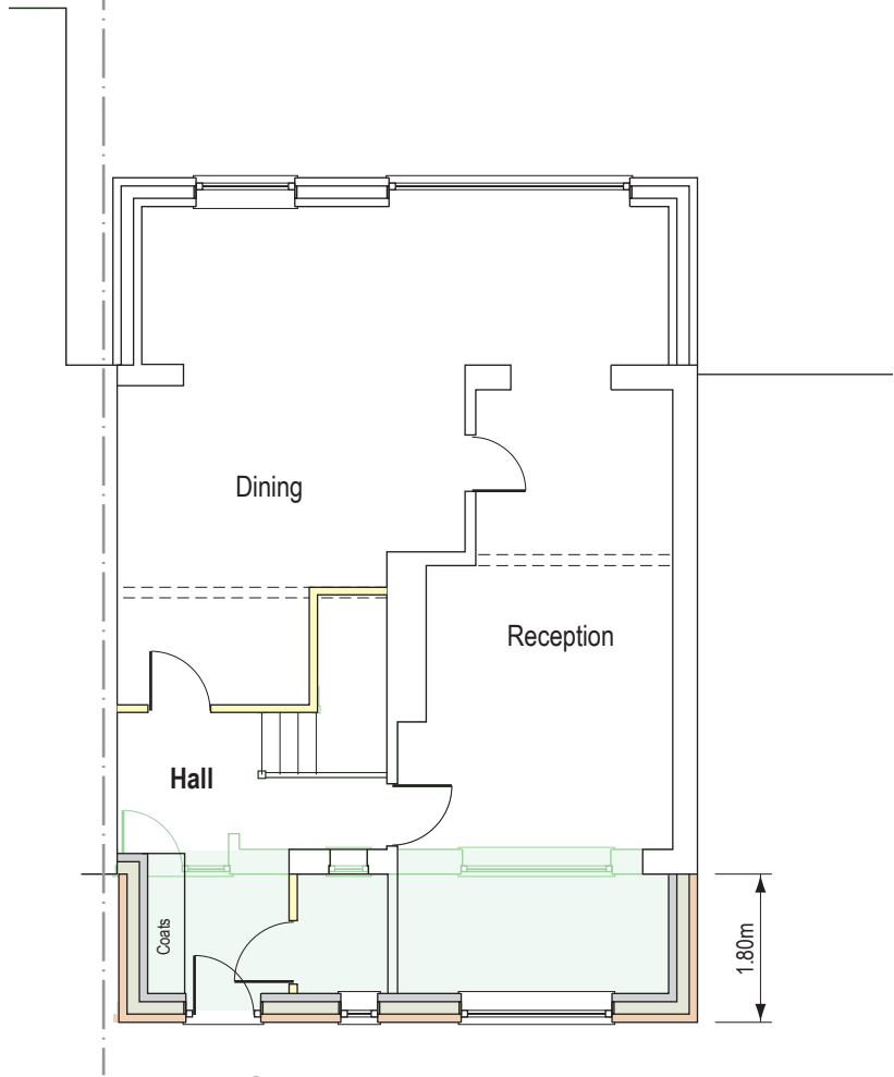
Ground Floor Plan (10.5m2)
