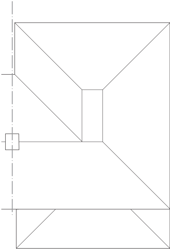
Roof Plan
