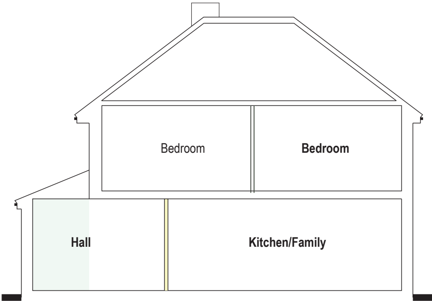
Section
