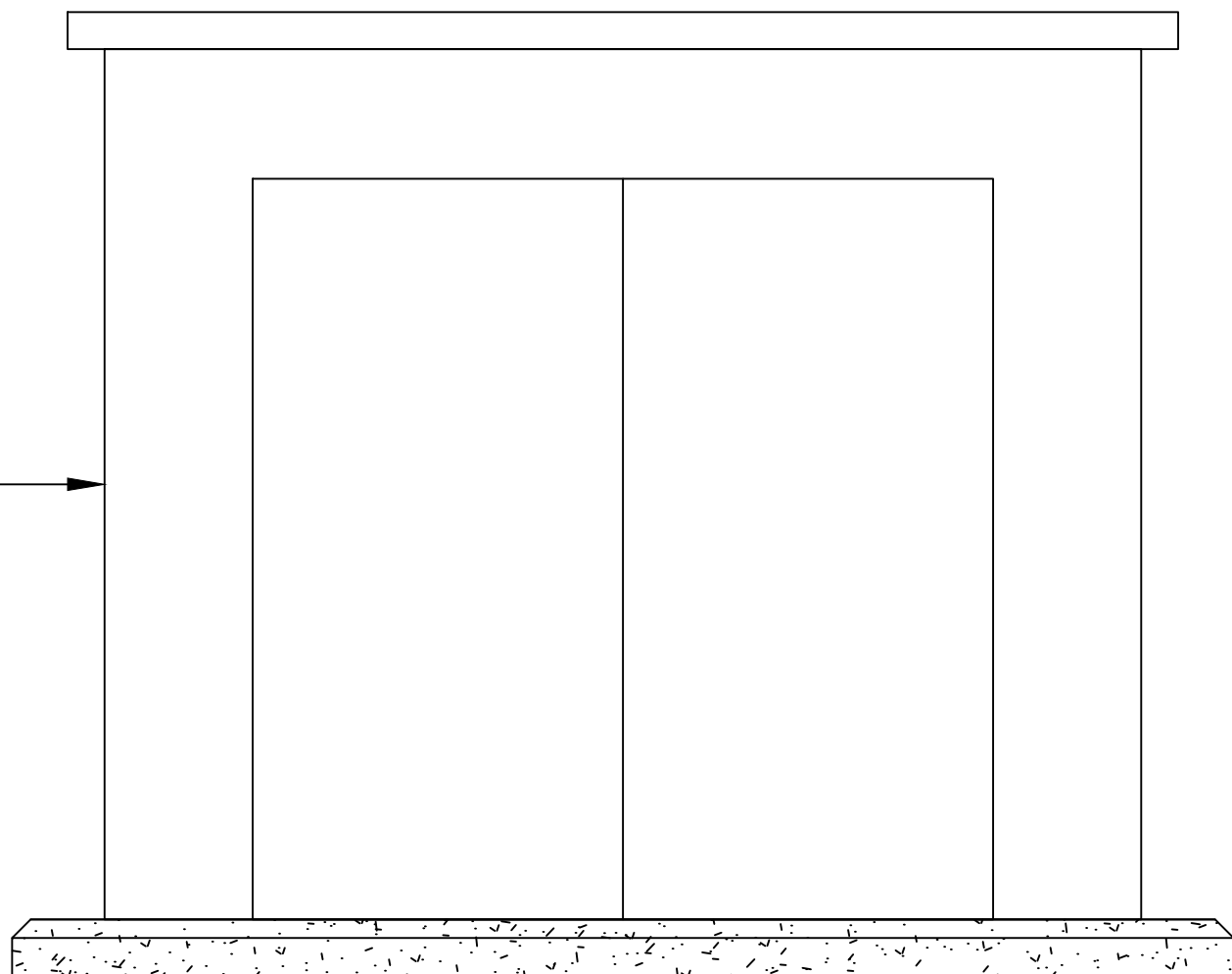
LV UNIT ELEVATION A - SOUTH SCALE - 1:20
