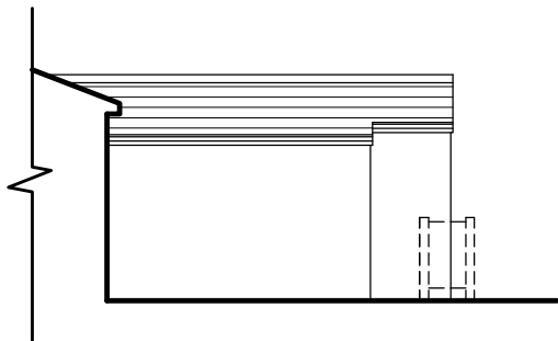
Elevation B @ 1/100
