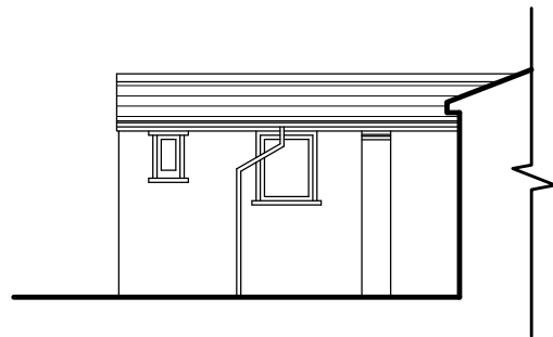
Elevation C @ 1/100
