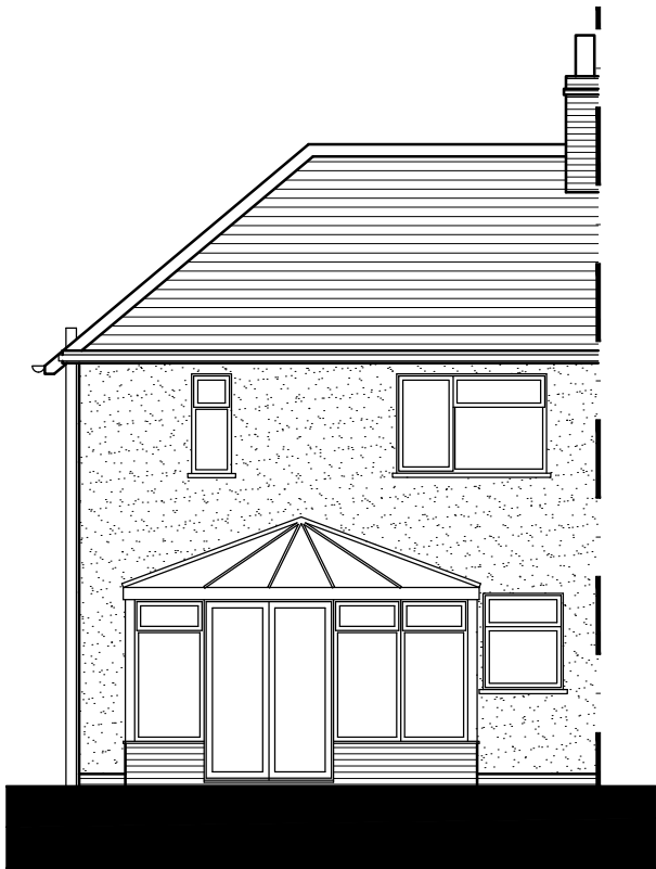
REAR ELEVATION (C-C)
