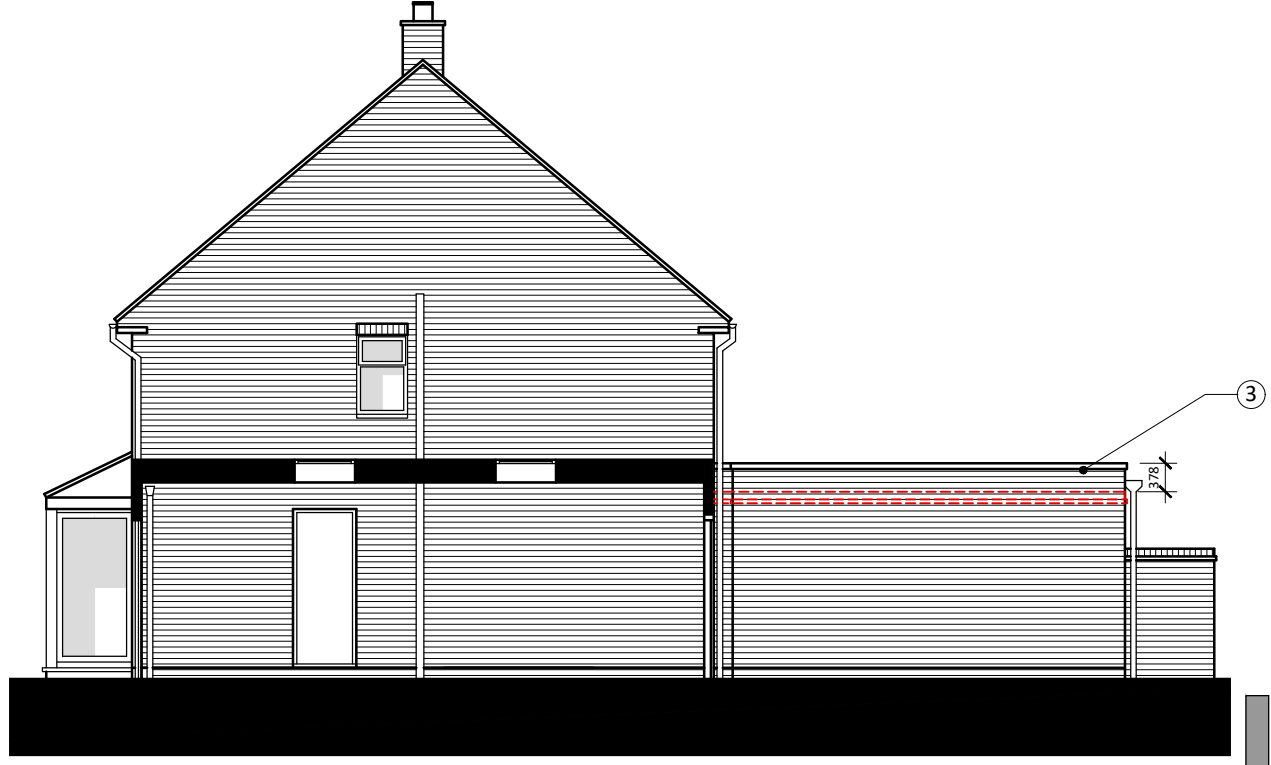
SIDE ELEVATION (D-D)
