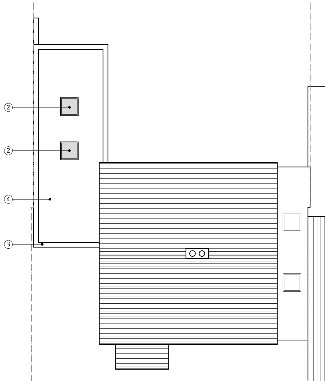
ROOF PLAN
