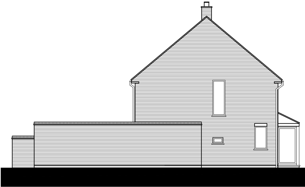
SIDE ELEVATION (B-B)
