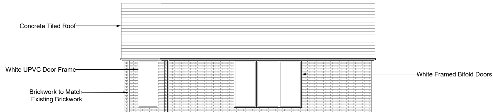
South Elevation
