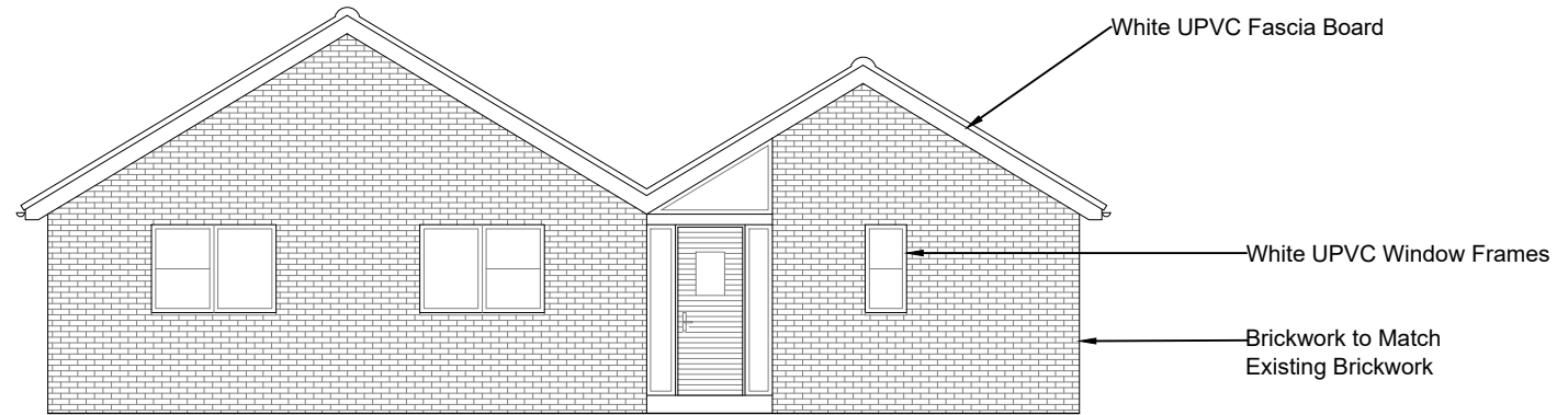
East Elevation
