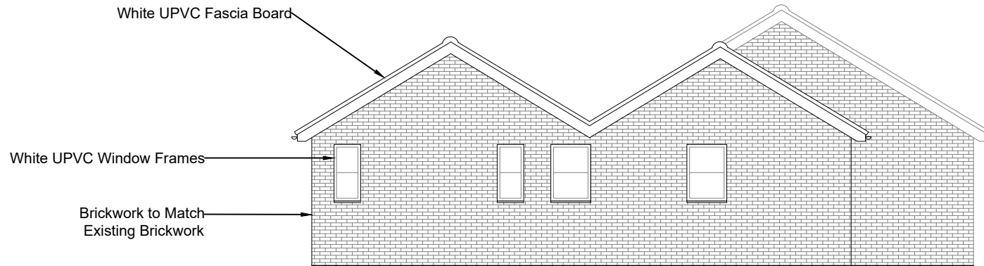
West Elevation
