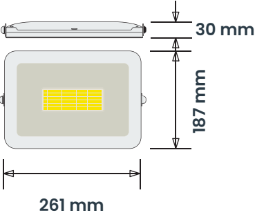
Floodlight Detail Scale 1:10
