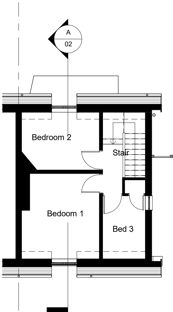
Existing First Floor Plan 1 : 100
