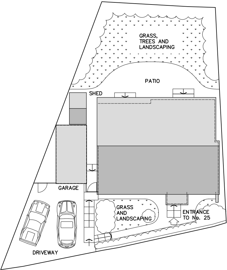
EXISTING SITE AND ROOF PLAN 1:200
