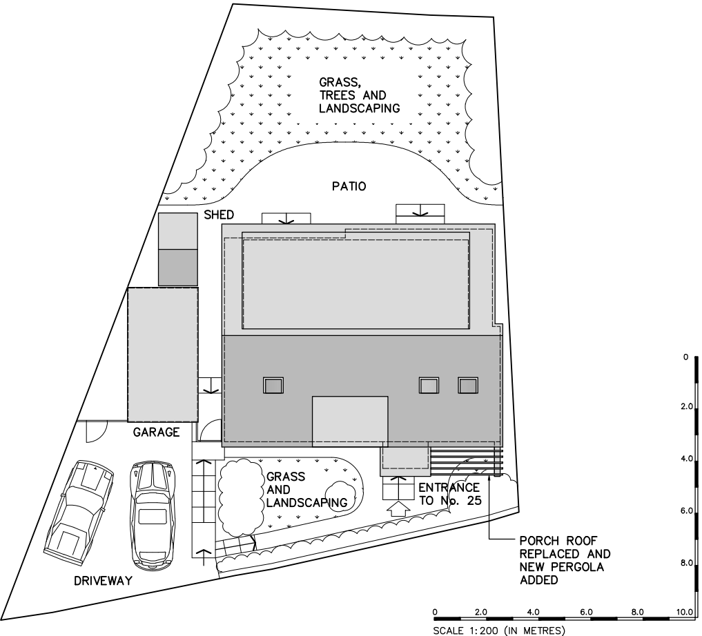
PROPOSED SITE AND ROOF PLAN 1:200
