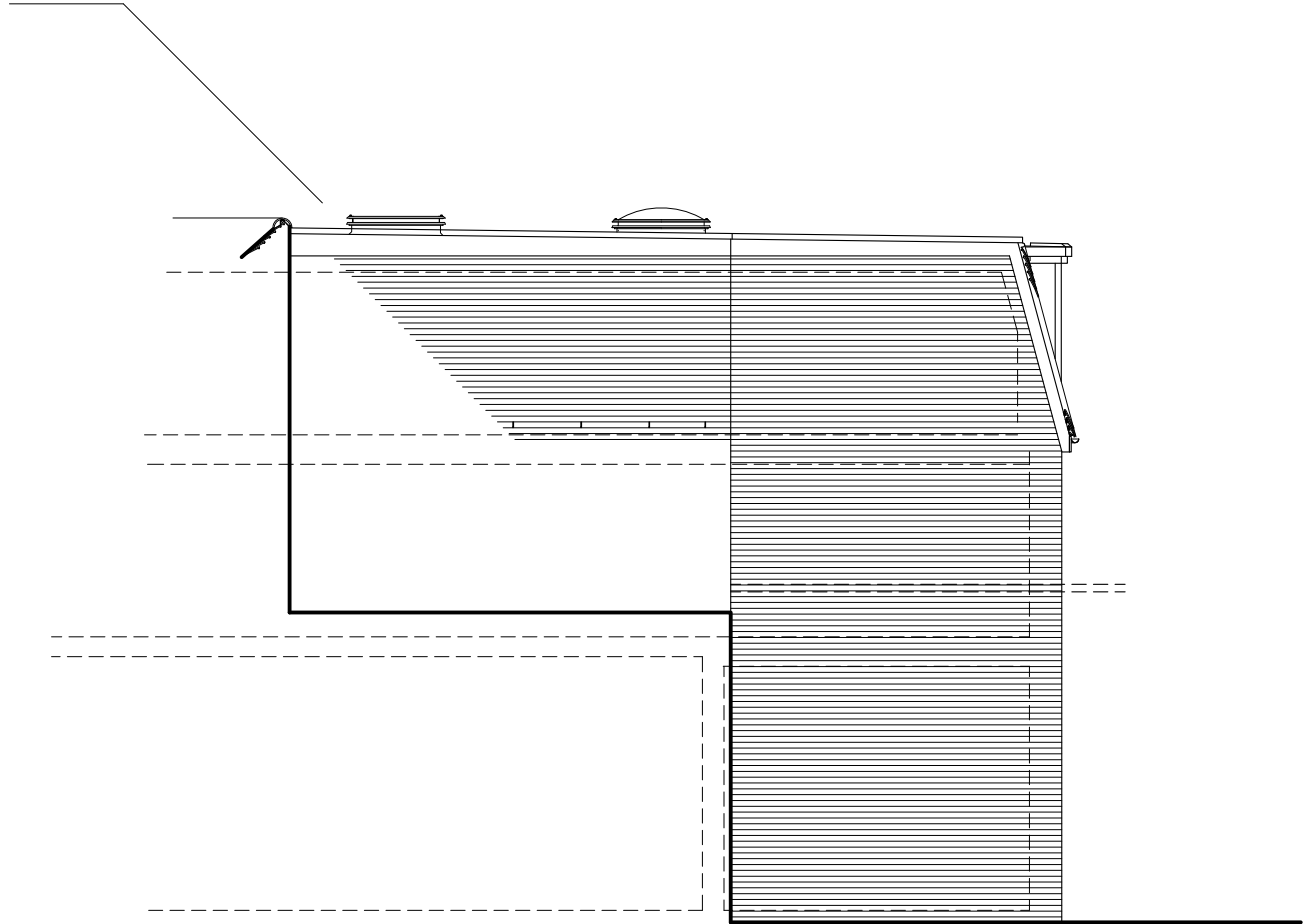
Existing Side Elevation (East)
