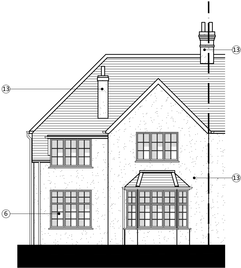
FRONT ELEVATION (A-A)
