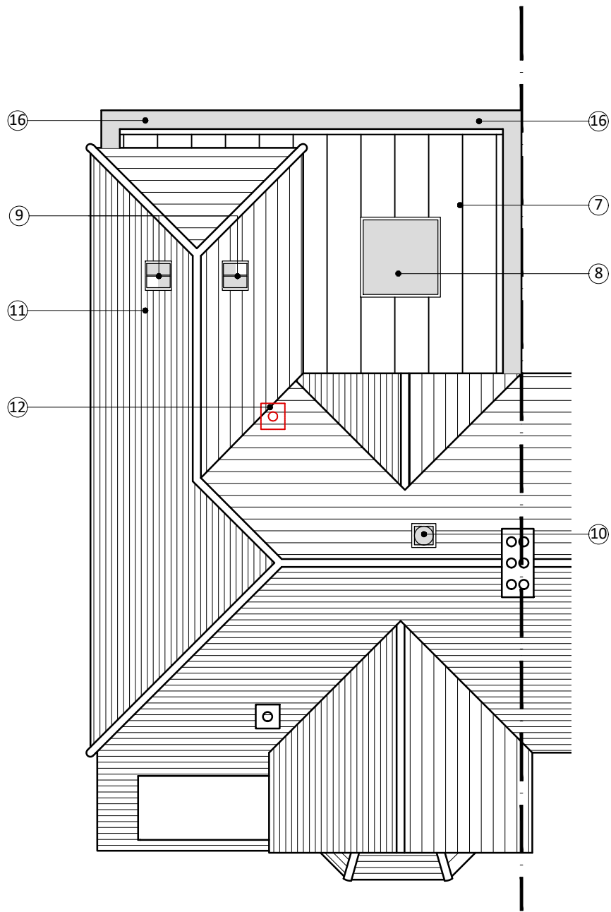
ROOF PLAN
