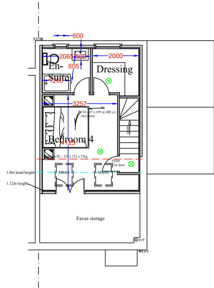
PROPOSED LOFT FLOOR LAYOUT
