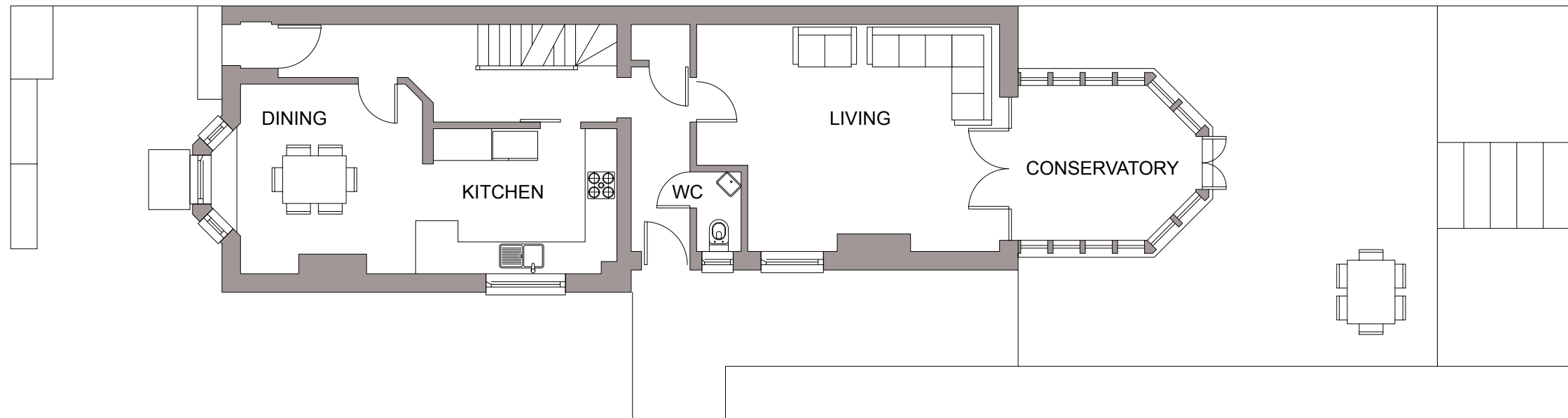
GROUND FLOOR
