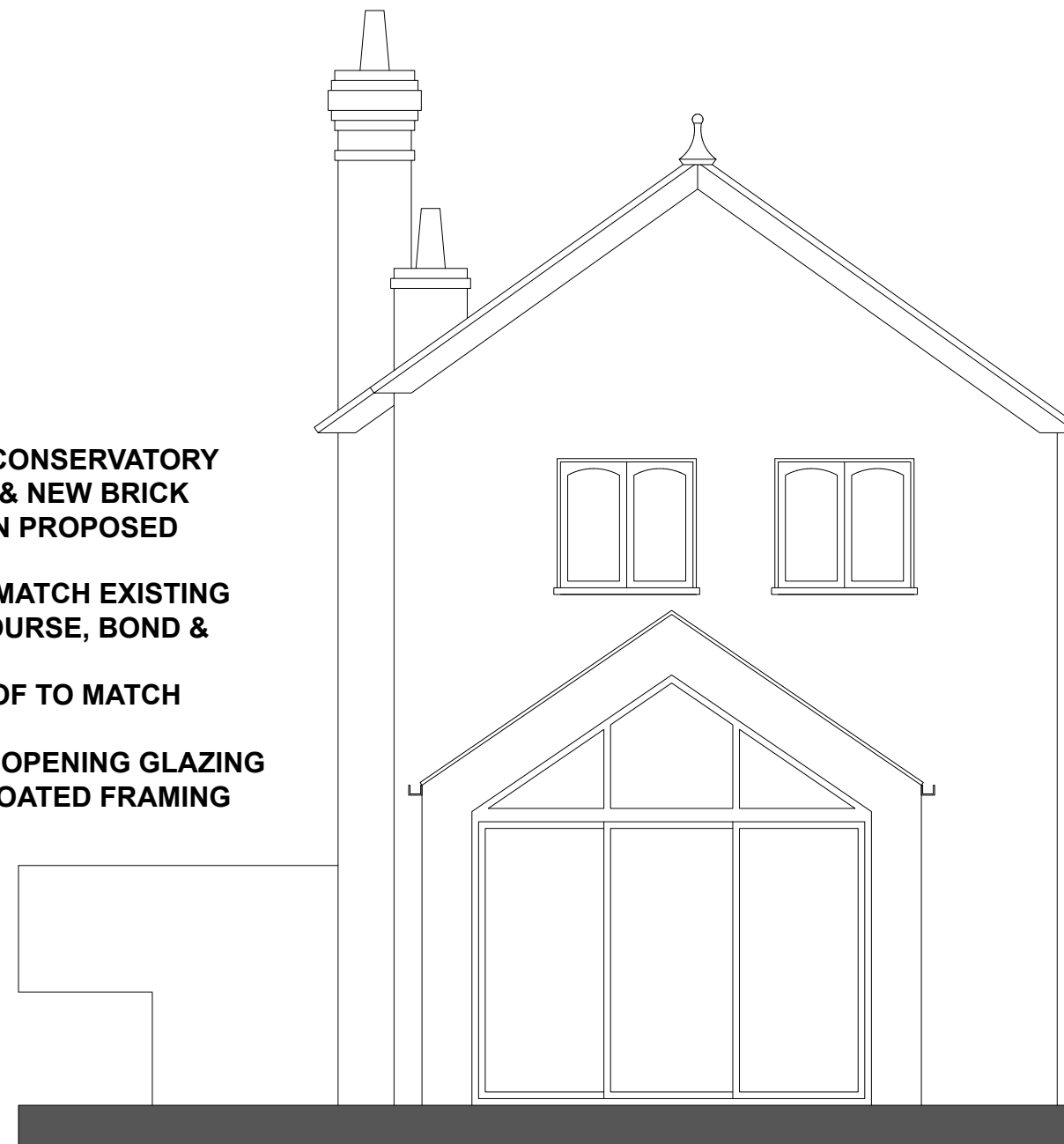
REAR ELEVATION
