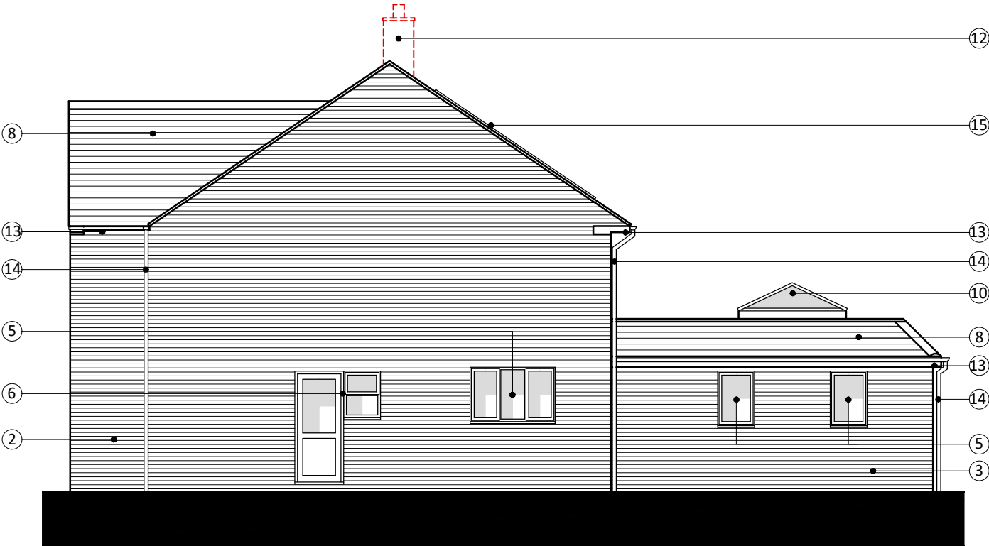
SIDE ELEVATION (D-D)
