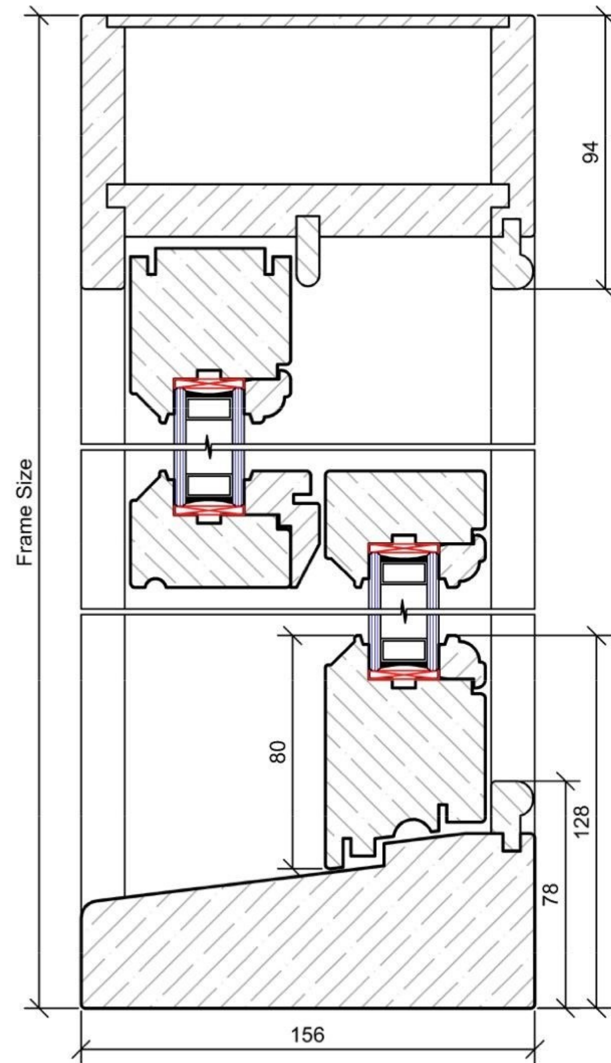
Vertical Section
