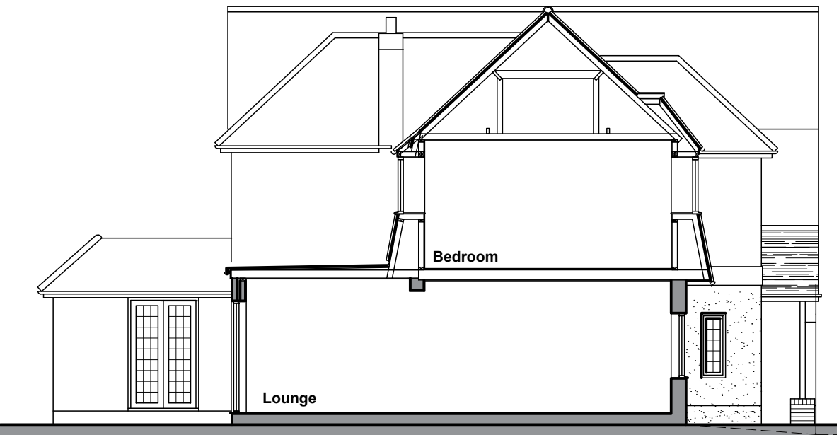
Existing Longitudinal Sections 1:100
