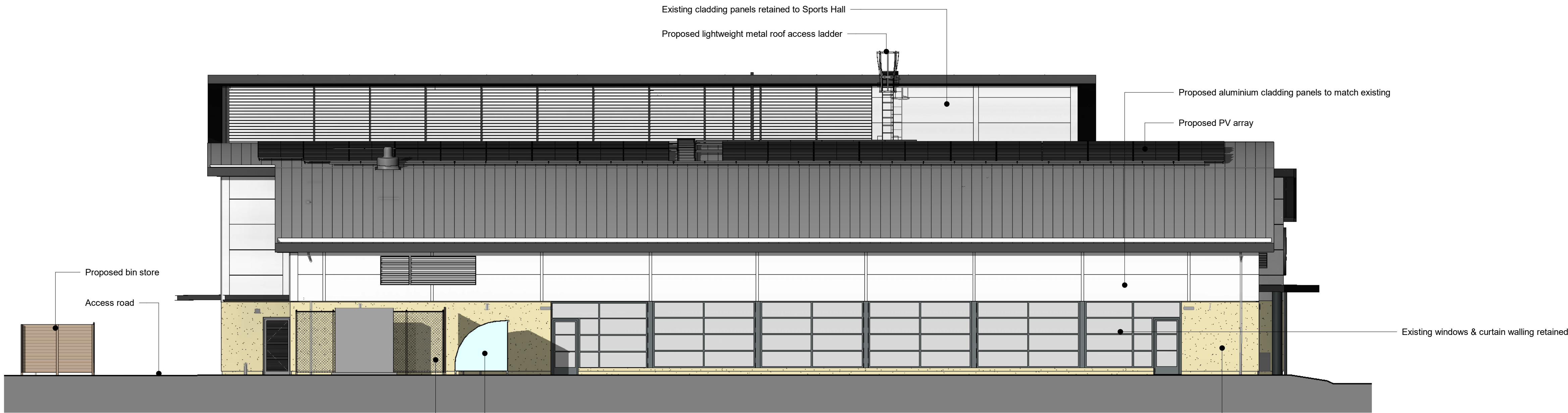
East Elevation - Proposed 1 : 100
