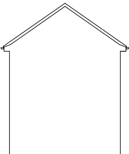
Building B Rear Elevation
