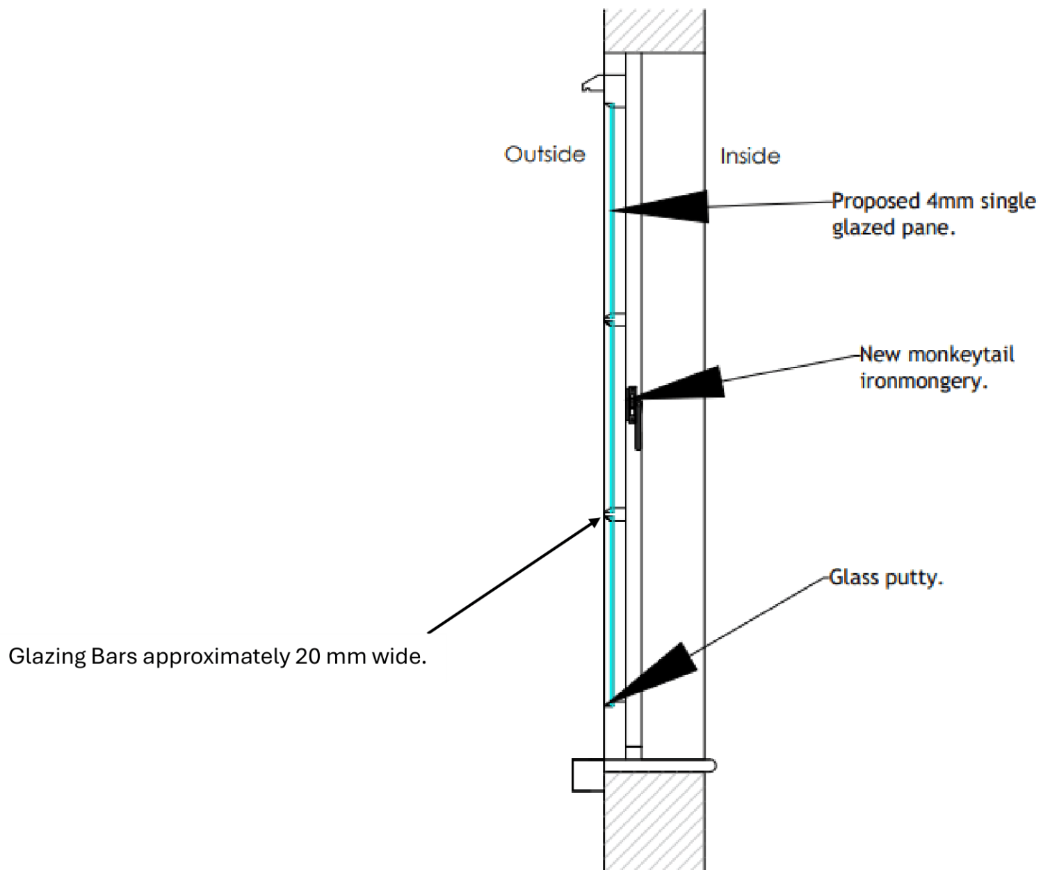
Figure 1 Section Drawing
