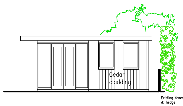
Front Elevation @ 1/100
