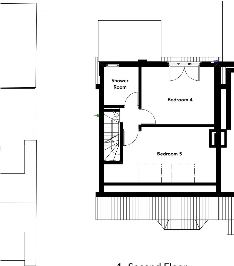
1. Second Floor 1:100
