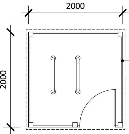
BIKE STORE PLAN
