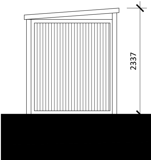
SIDE ELEVATION (B-B)
