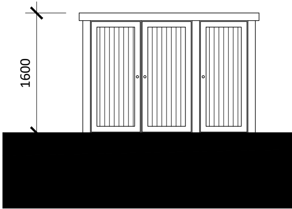
FRONT ELEVATION (A-A)
