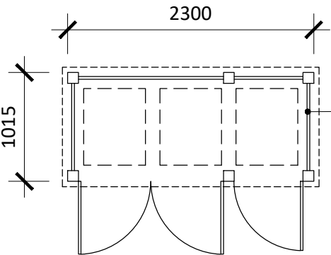
BIN STORE PLAN
