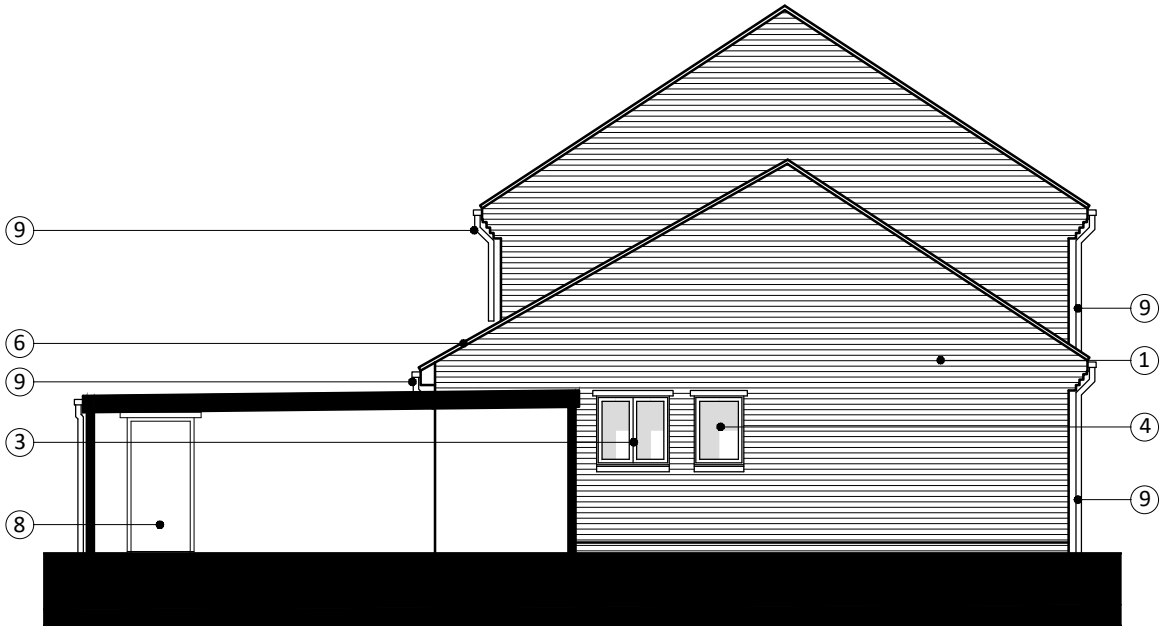
SIDE ELEVATION (D-D)
