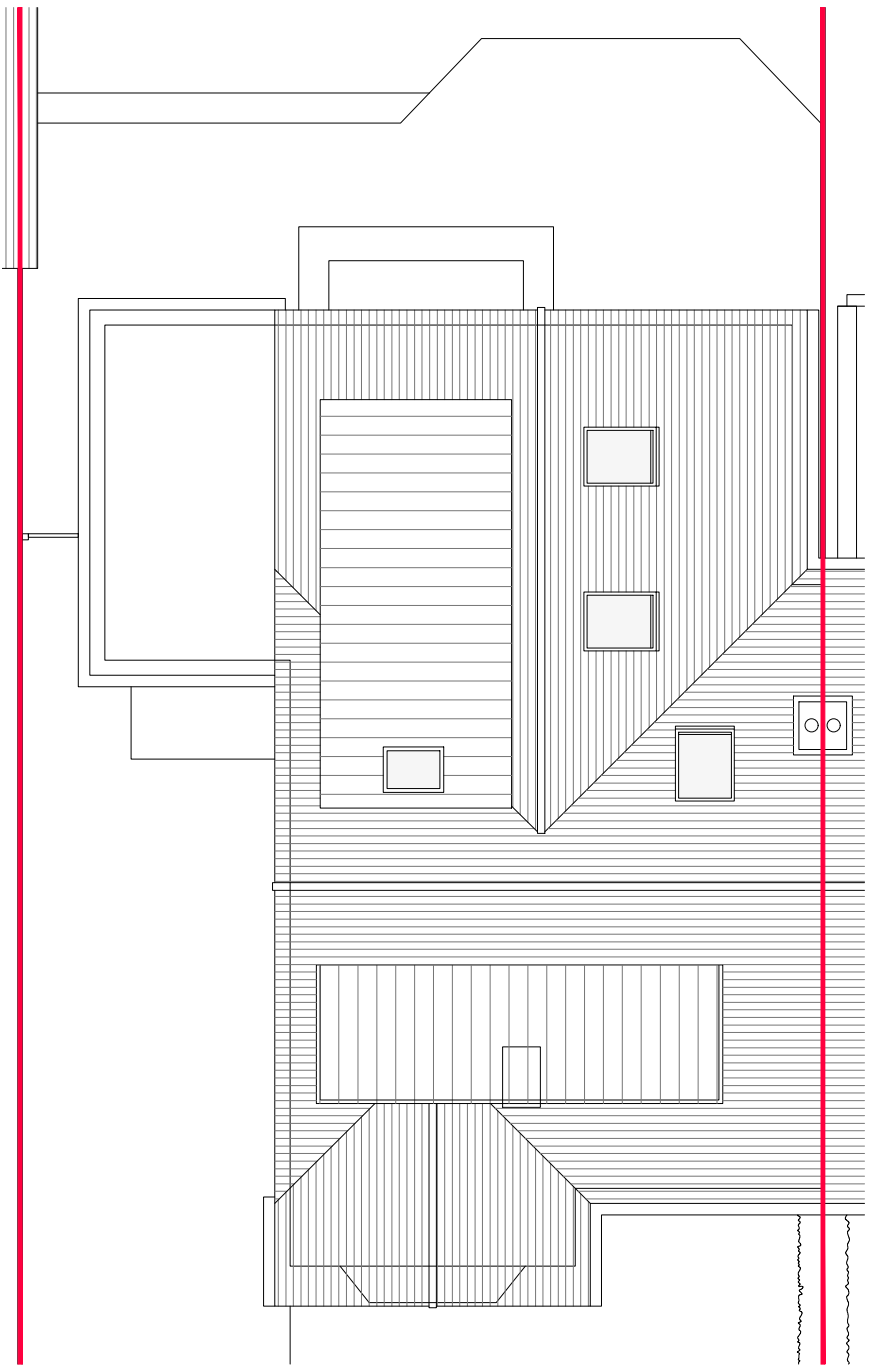
ROOF PLAN (1:100)
