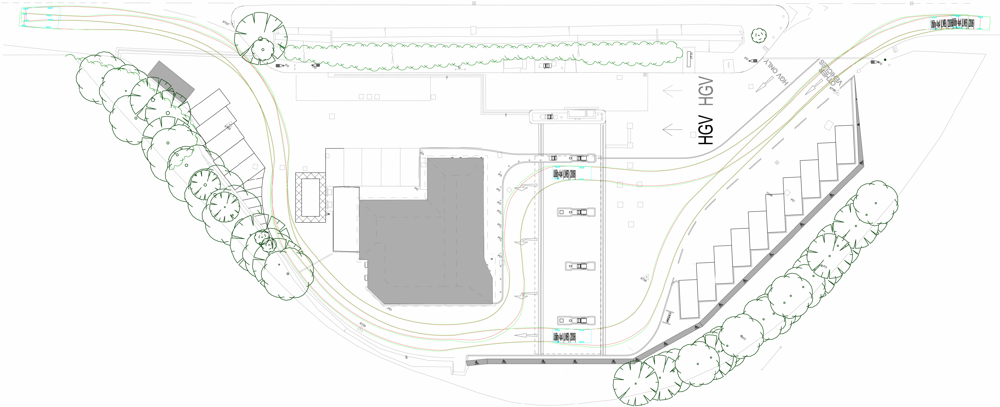
LWB 4x4 Fuel Purchase Route 1 : 250
