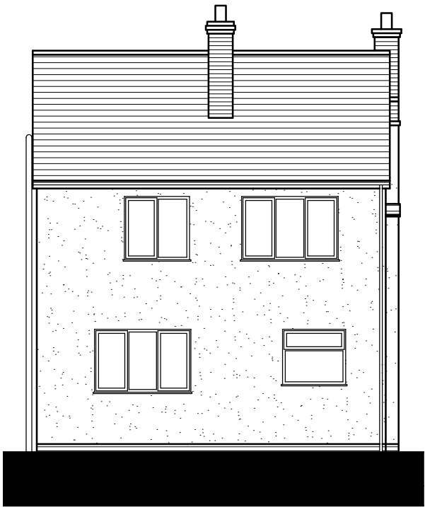
REAR ELEVATION (C-C)
