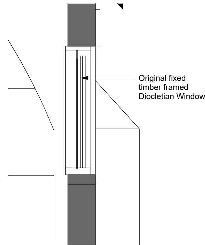
3 Existing - Diocletian Window - Section 1 : 25
