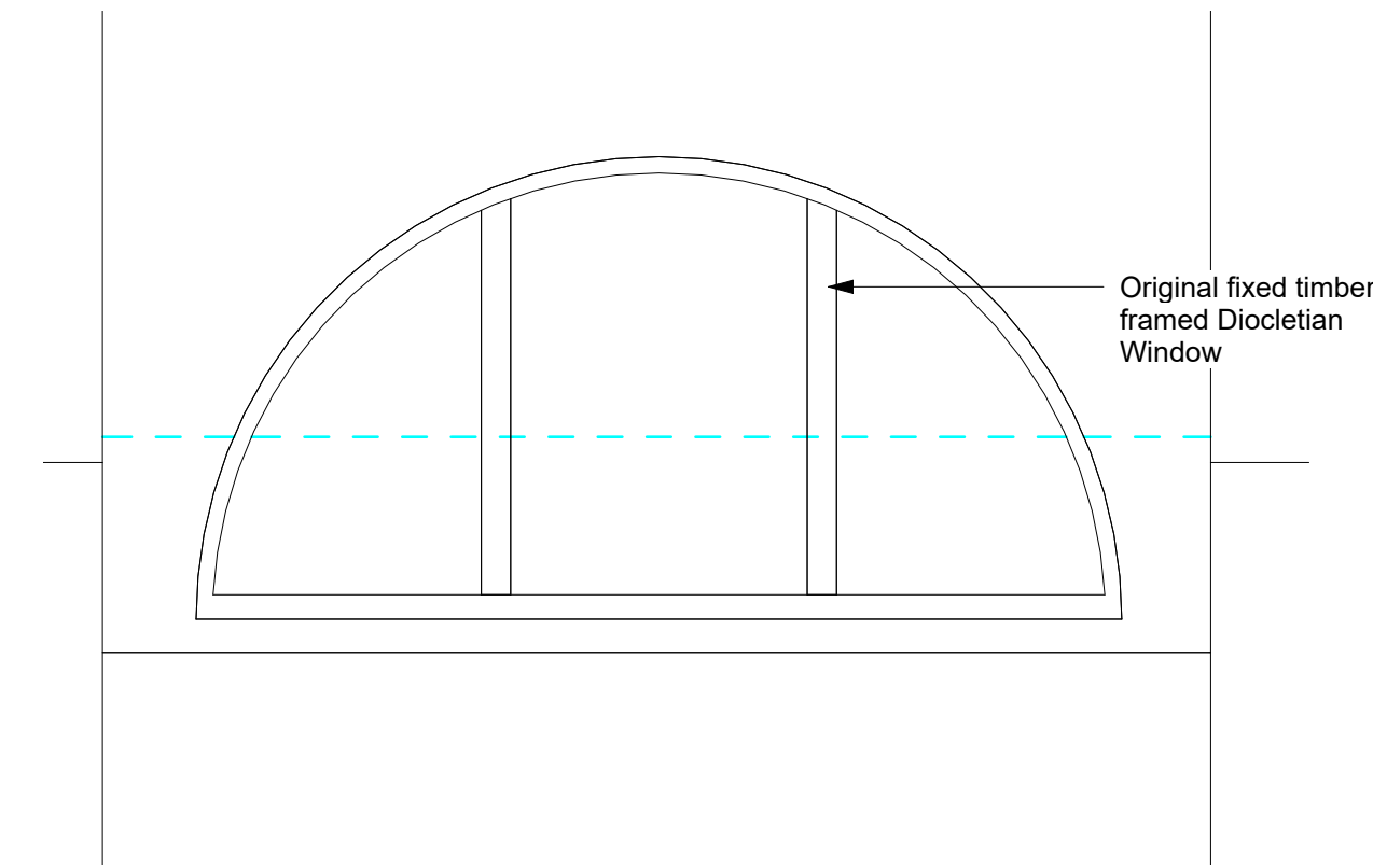
4 Existing - Diocletian Window - Elevation 1 : 25
