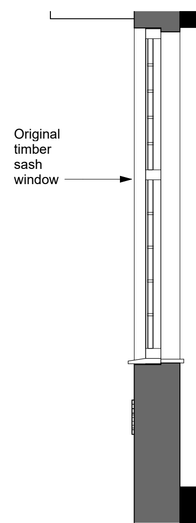
5 Existing - Sash Window - Section 1 : 25
