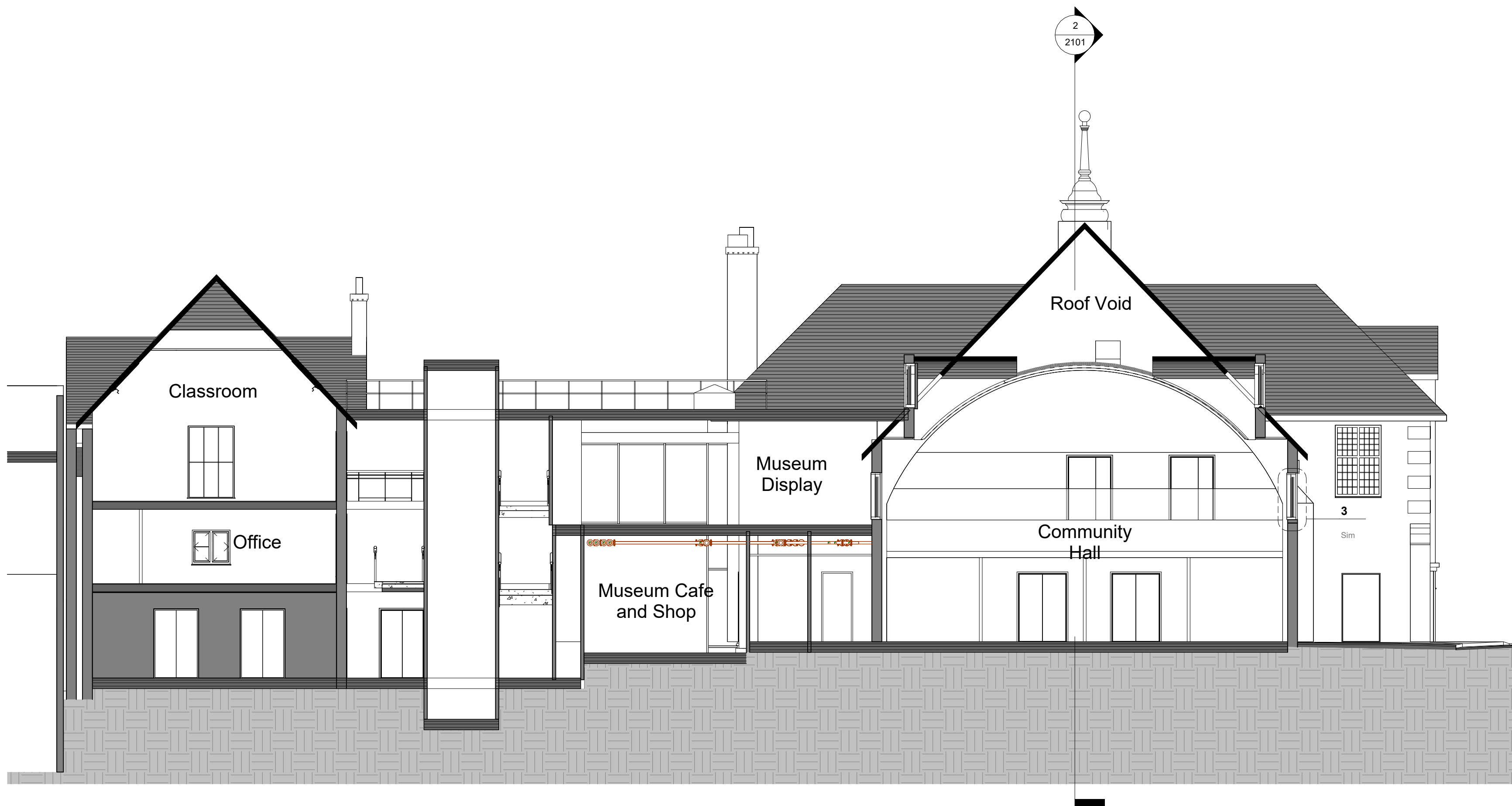
1 Existing - Cross Section 1 : 100
