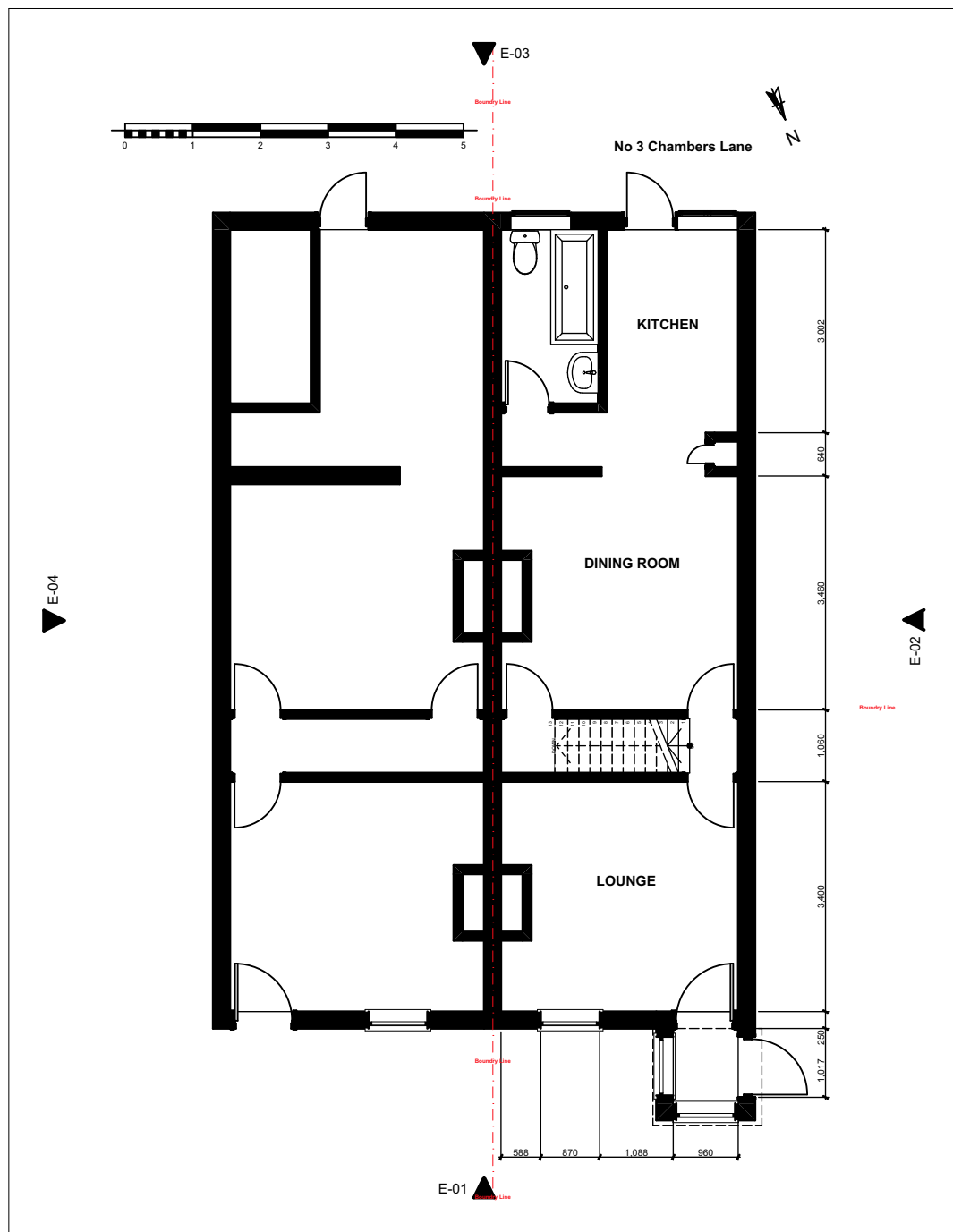
A-001 GROUND FLOOR EXISTING 1:100
