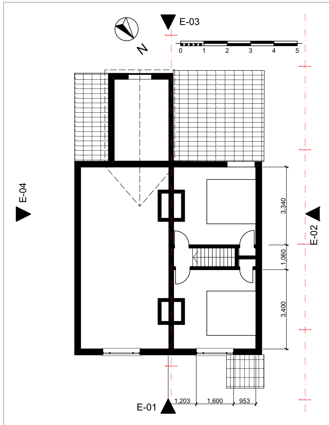
A-002 FIRST FLOOR EXISTING 1:100
