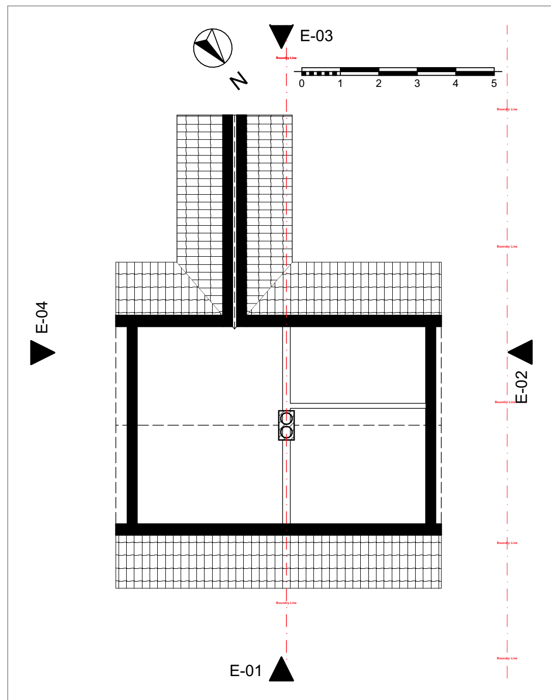
A-003 ROOF EXISTING 1:100
