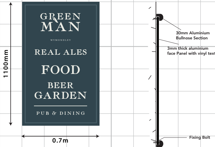
C FOUR X NEW AMENITY SIGNS (TWO FIXED BACK TO BACK ON POST) SIZE. 0.7m x 1100mm. H.A.G. 0.9/1.4m.
