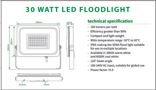
G FIVE X LED FLOOD LIGHTS SIZE. 0.23m x 168mm. H.A.G. 3.5/3.4m.
