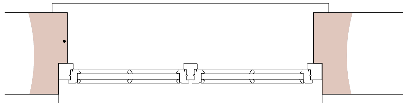
PLAN
