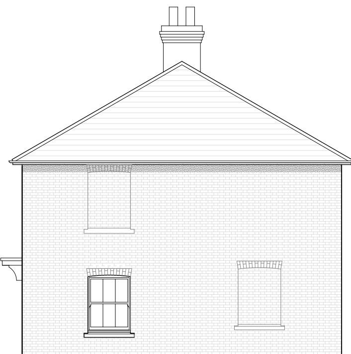
SOUTH ELEVATION 1:100
