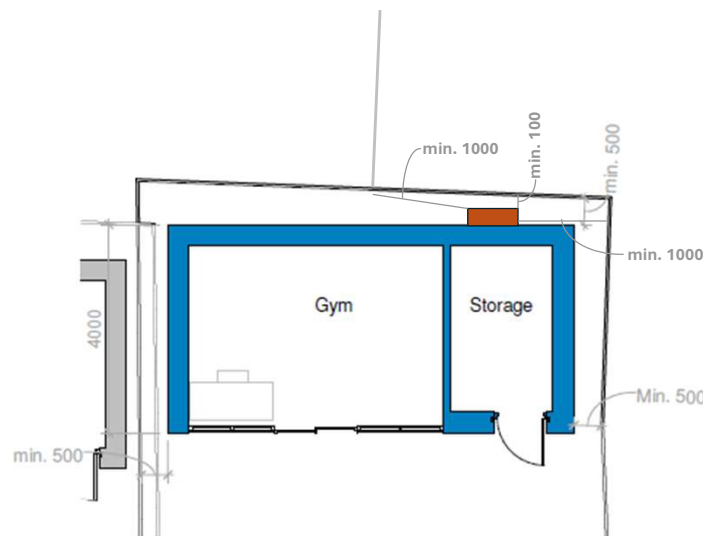
Proposed Garden Room Plan 1 : 100
