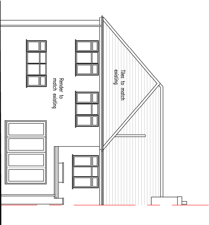
Rear Elevation @ 1/100
