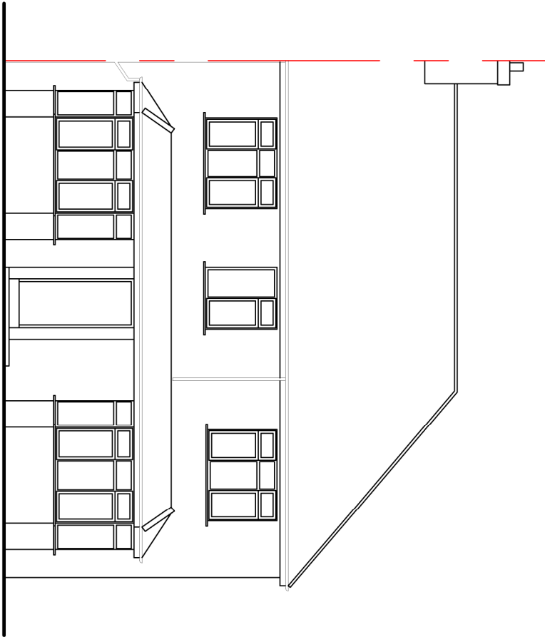
Front Elevation @ 1/100
