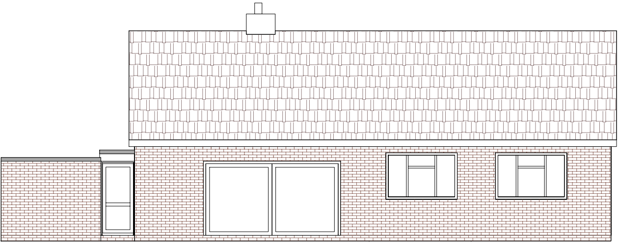
Existing Rear (West) Elevation 1:100 Scale
