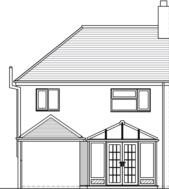
REAR ELEVATION
