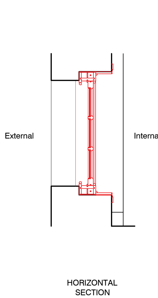
STAIRWELL WINDOW SECTIONS (W2) (1:20)
