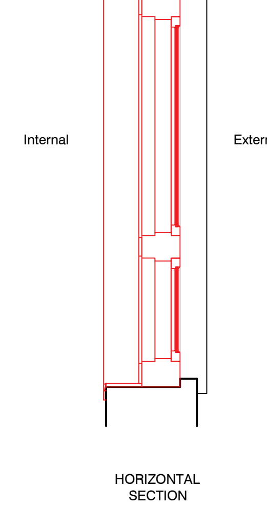
LOUNGE/DINING ROOM WINDOW SECTIONS (W4) (1:20)
