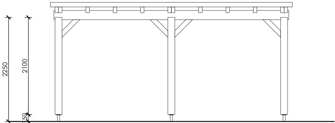
Carport - Side Elevation
