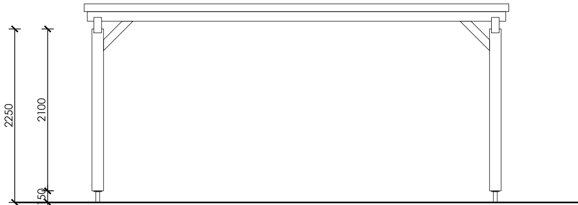
Carport - Front Elevation
