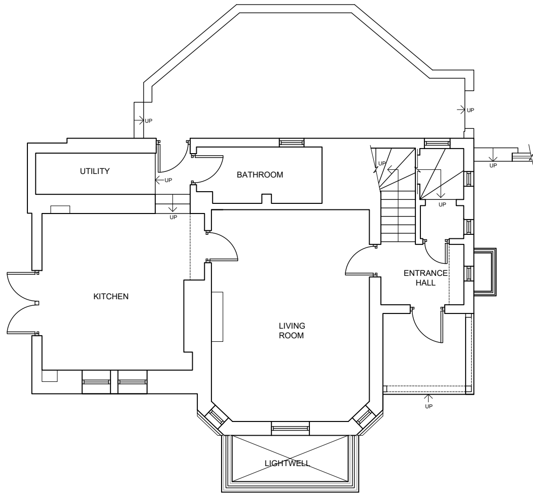
PROPOSED GROUND FL PLAN - UNITS 16 & 17
