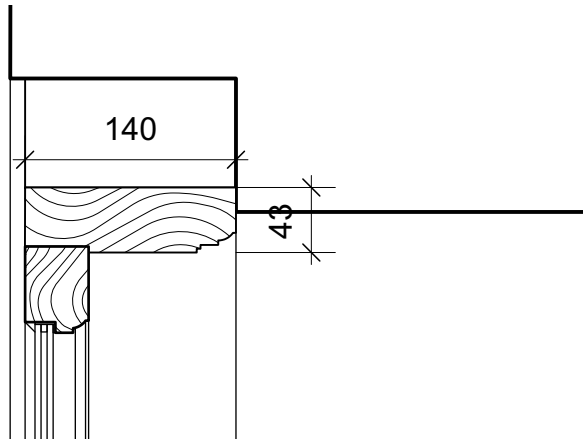
○ Typical Head Detail - Section Scale 1:5
