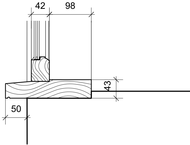
○ Typical Sill Detail - Section Scale 1:5
